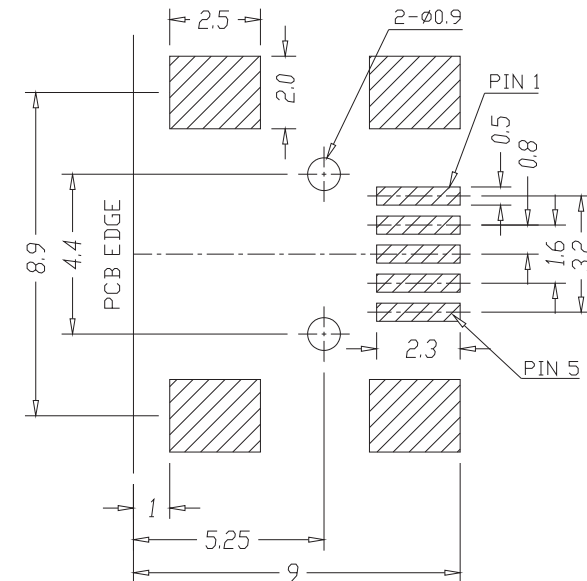
RECOMMENDED PCB PATTERN LAYOUT (PCB THICKNESS:0.8±0.1)
